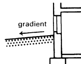
10 Paths beside house
